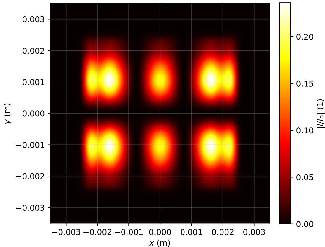
Intensity profile I(x, y, z = 3.821)/I_0 , P_{in}=0.5P_{cr} , artificial time
